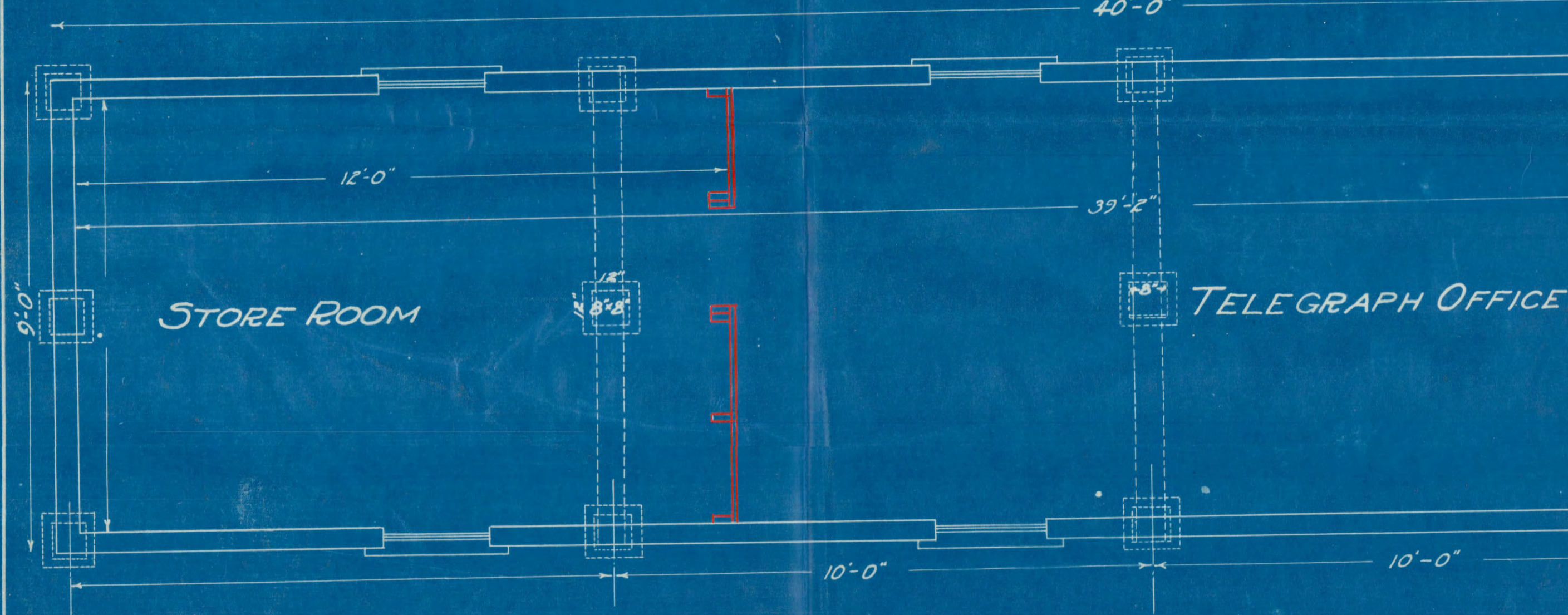
PLAN Arrangement of Piers Scale \frac{1}{2} = 1
