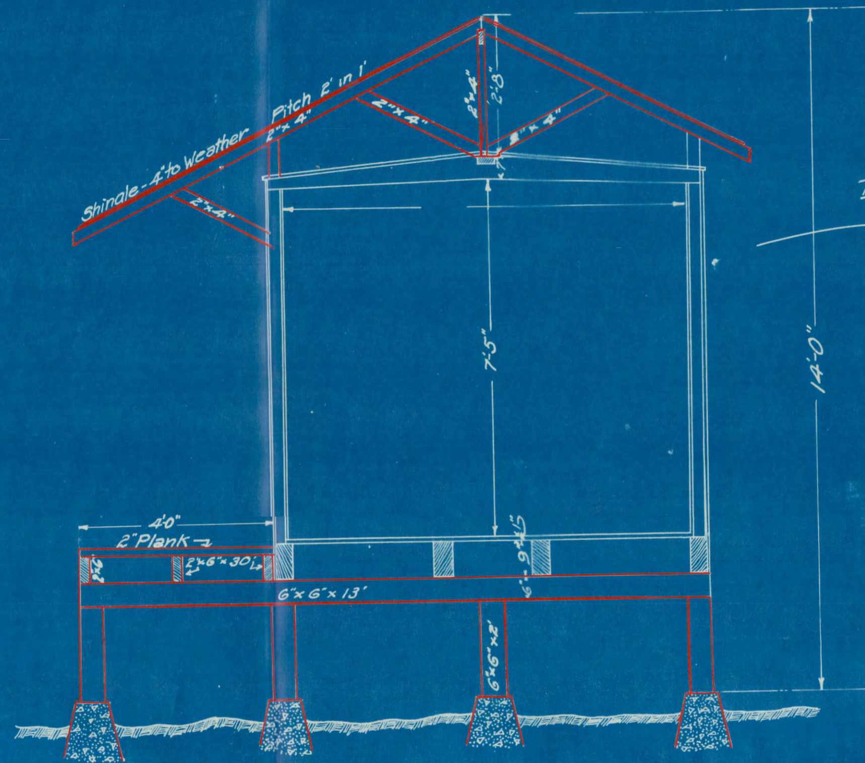
SECTION A-A Scale \frac{1}{2} = 1
